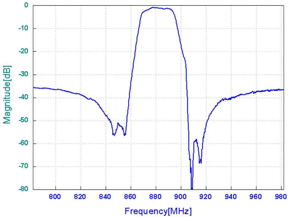
Frequency Response
